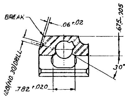
SECTION H-H
