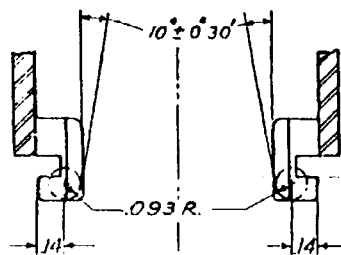
PARTIAL SECTION E-E SCALE \frac{2}{1}
