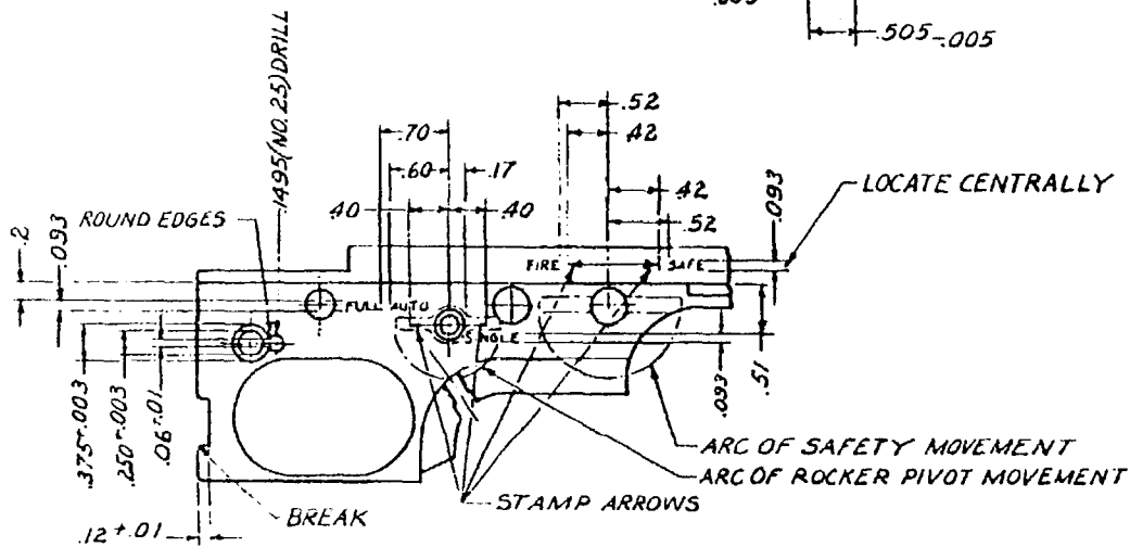
DETAIL SHOWING MARKING TO BE STAMPED ON FRAME
