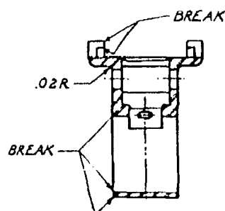
SECTION F-F
