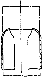
SECTION A-A WITH FORMING TOOL
