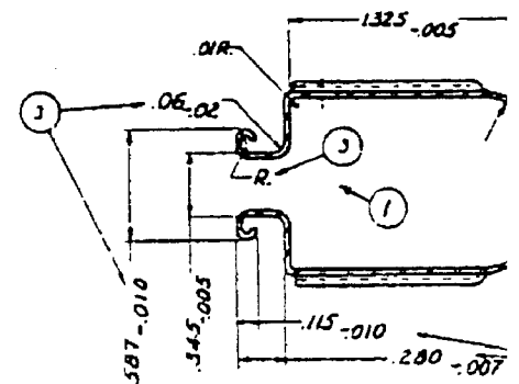
SECTION C-C SCALE \frac{2}{1}
