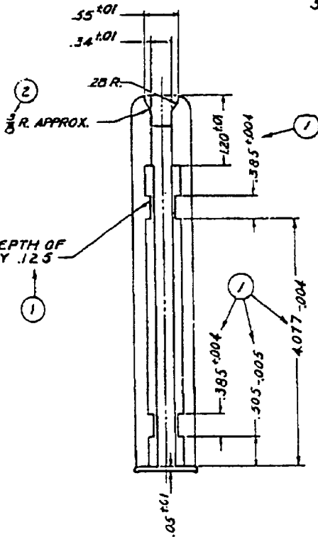
SECTION A-A WITH FORMING TOOL
